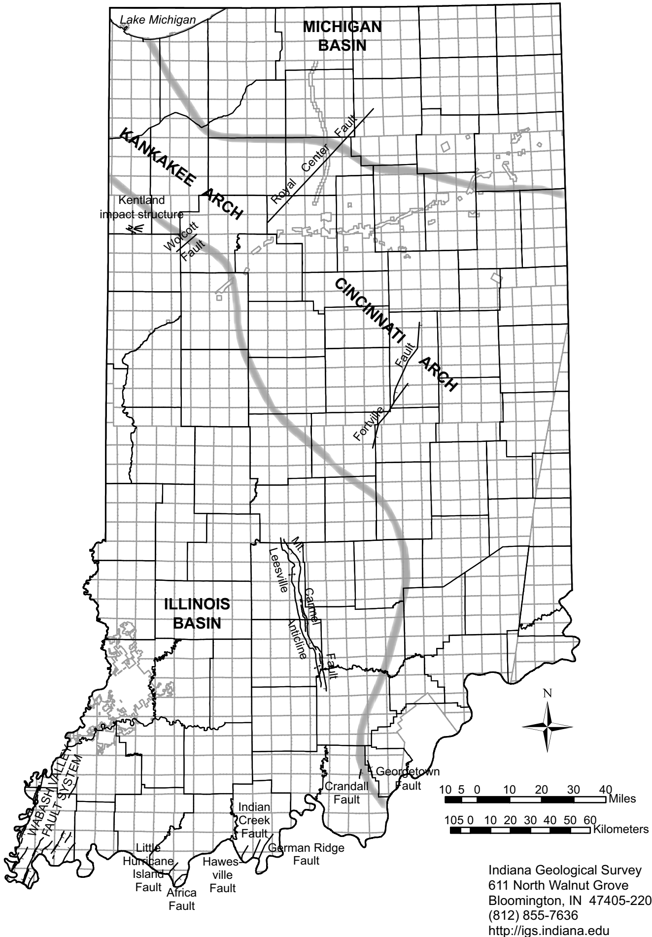
Map of Indiana Showing Major Geologic Structures
